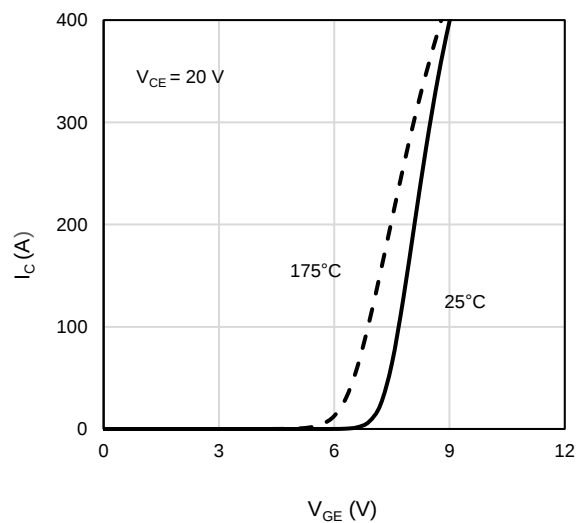
Figure 6: Transfer Characteristics
