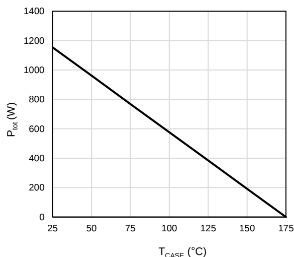
Figure 2: Power De-rating
