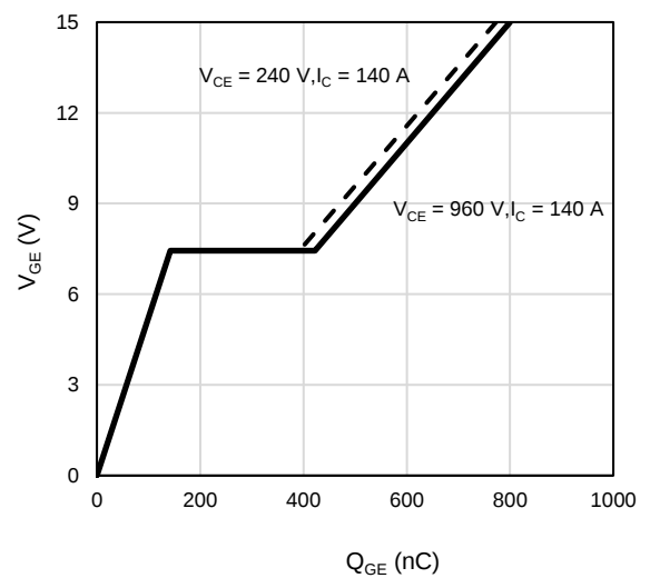
Figure 16: Gate-Charge Characteristics
